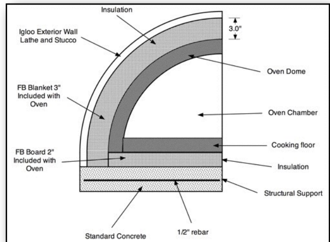
9.1 The sections of an Igloo oven.
