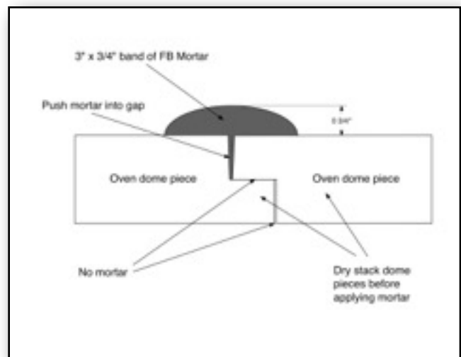
5.3. Dome assembly.
