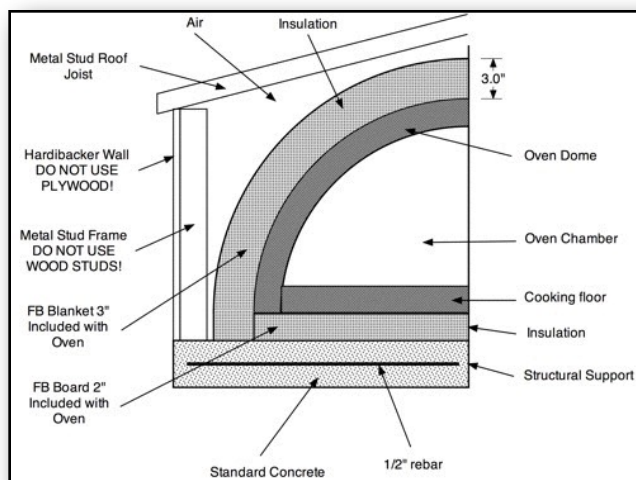
10.1. The basic walled enclosure.
