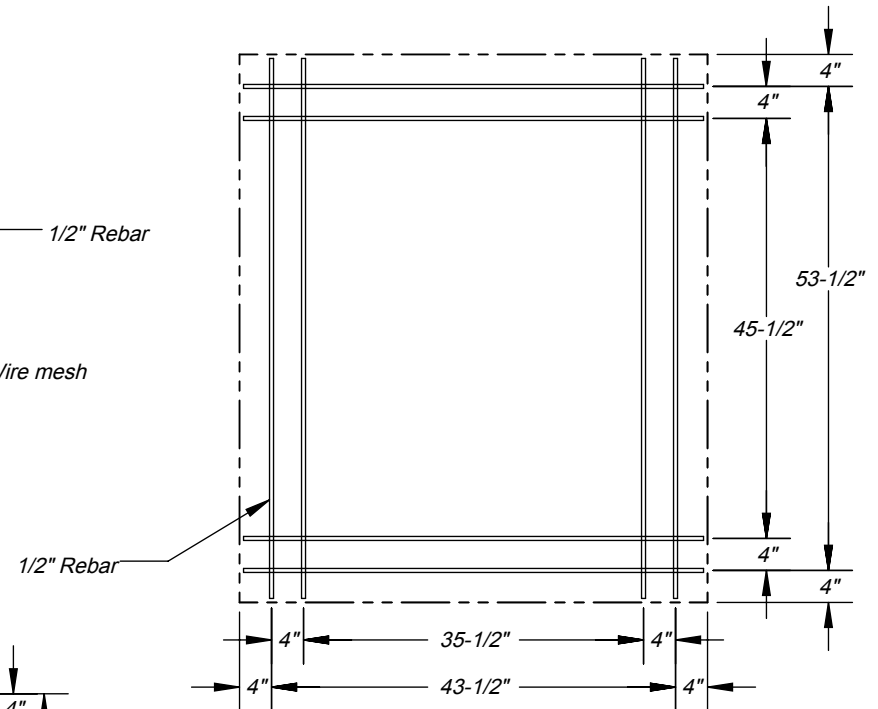
Cucina 70W oven stand footprint (*See specifications for CMU stand)
