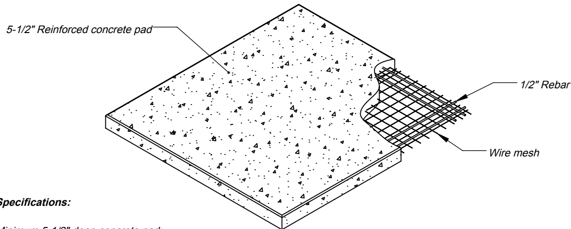
Cucina 70W oven stand footprint (*See specifications for CMU stand)
