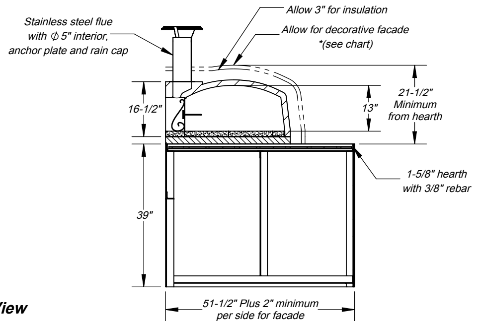
Side Elevation
