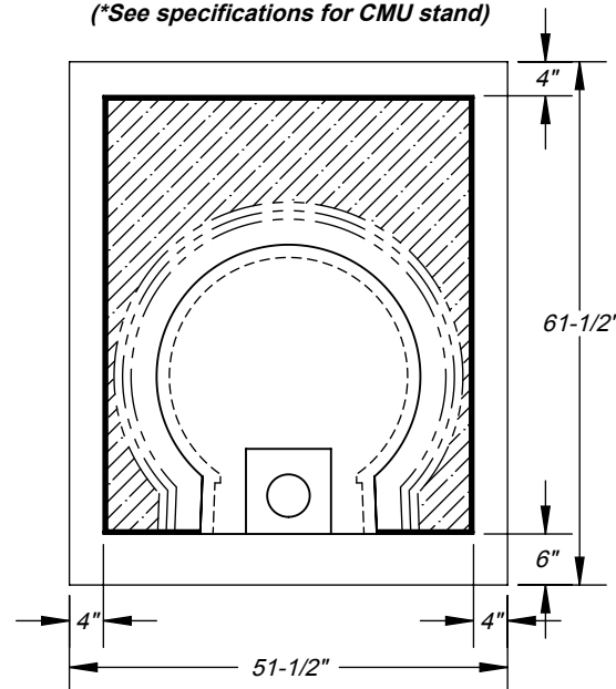
Cucina 70W oven stand footprint (*See specifications for CMU stand)
