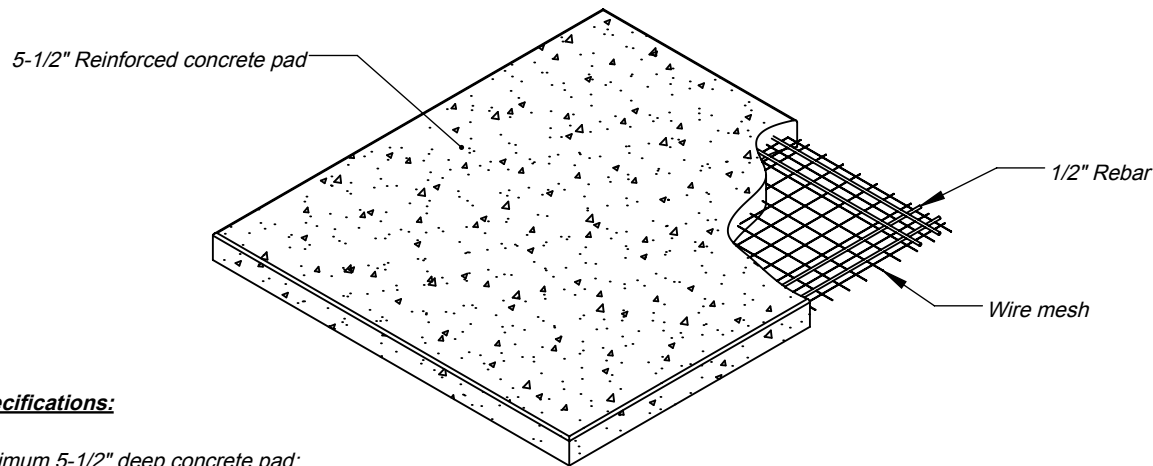
Cucina 120 oven stand footprint (*See specifications for CMU stand)
