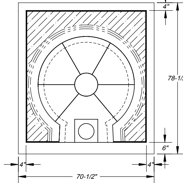
Cucina 120 oven stand footprint (*See specifications for CMU stand)
