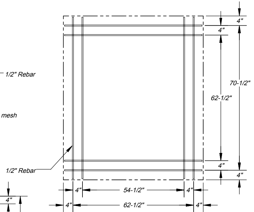
Cucina 120 oven stand footprint (*See specifications for CMU stand)
