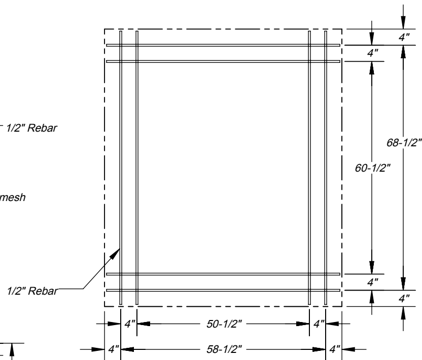
Cucina 110 oven stand footprint (*See specifications for CMU stand)
