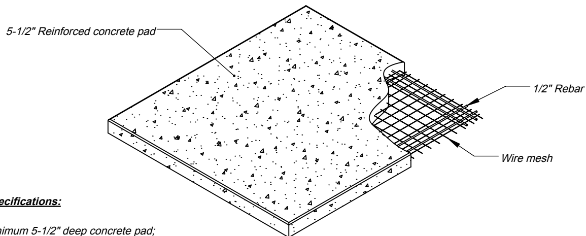
Cucina 110 oven stand footprint (*See specifications for CMU stand)
